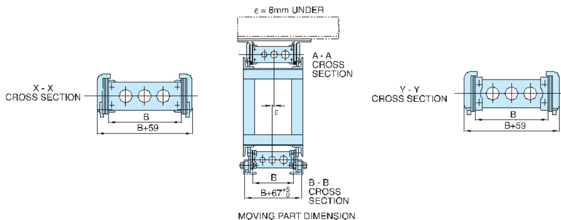
MOVING PART DIMENSION
