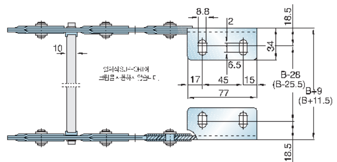
Moving Bracket
