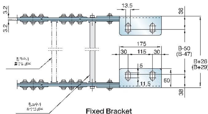
Fixed Bracket
