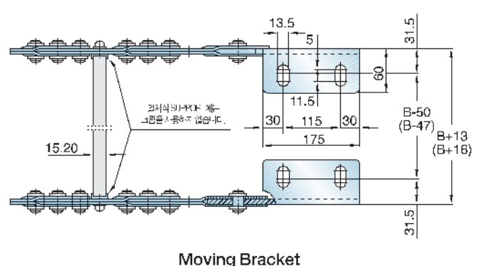
Moving Bracket
