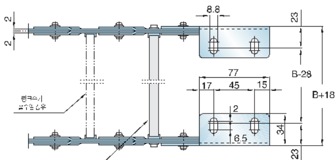
Fixed Bracket
