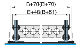
Guide Rail
